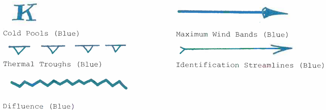
Figure 32. LFM 500 mb Vorticity Panel (12-hour Prognosis).
